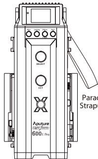
LS 600x Pro Control Box (1 pc)
