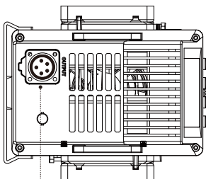
5-Pin Female Head Cable Connector
